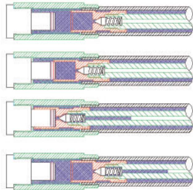
KAM® IAS™ sampler pumping sequence
