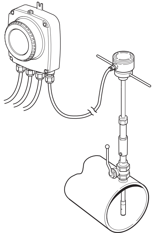
Fig. 3: FEA100 remote system
